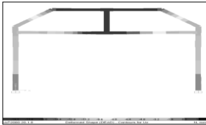
F24. Structure displacement diagram under dead load.
