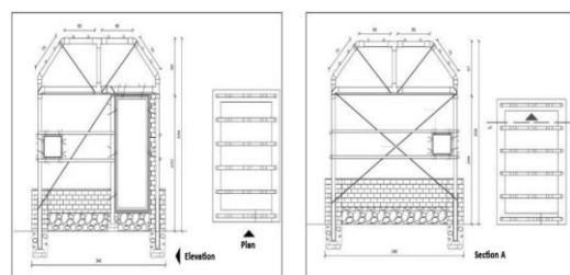
West elevation
